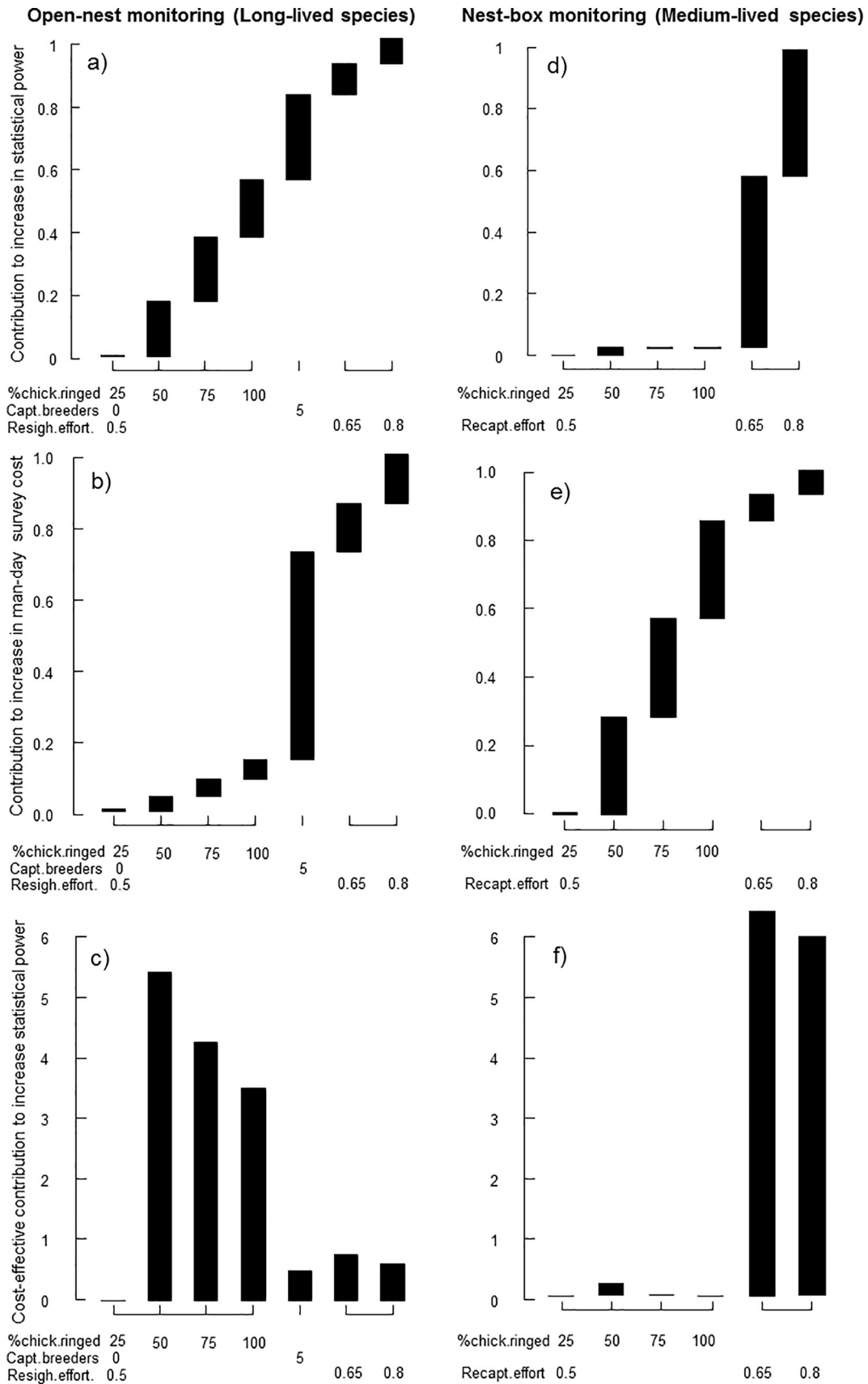
Fig. 4. Relative contribution to the increase in statistical power (a,d) and cost (b,e), and cost-effective contribution (c,f) of different components of capture-recapture design (proportion of chicks ringed [%chick.ringed], capture of breeding birds for ON monitoring only [Capt.Breeders], effort dedicated to resighting [Resigh.effort] or recapture [Recapt.effort] respectively for ON and NB monitoring). The survey reference was the short-duration one (5 years for NB, 10 years for ON) and 50 and 75 surveyed pairs, respectively for ON and NB.
